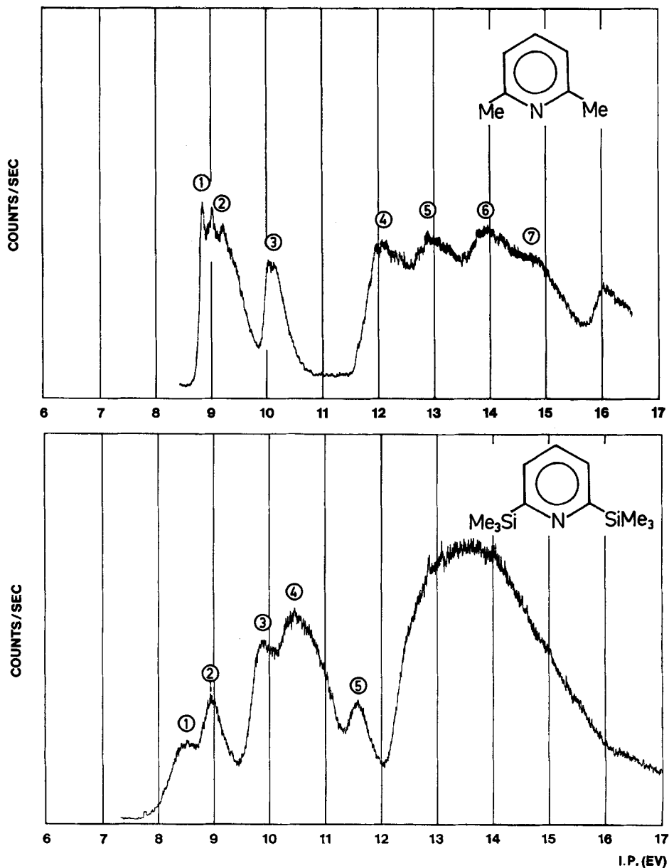
Figure 1. PE-spectra of 2,6-dimethylpyridine (V) and 2,6-bis-trimethylsilyl-pyridine (IX).
